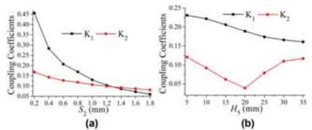
FIGURE 17. (a) The coupling coefficients of the first two modes against S_2 . (b) The coupling coefficients of the two modes against H_5 .
