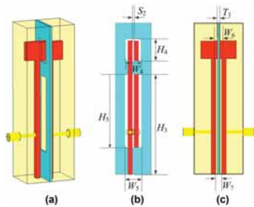
FIGURE 16. Coupling structure. (a) Three-dimensional view. (b) Left side view. (c) Front view.
