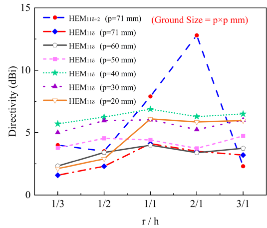
Fig. 3. Variation of antenna directivity with r/h operating in \text{HEM}_{11\delta+2} mode and \text{HEM}_{11\delta} mode at 8 GHz frequency. For the fundamental mode ( \text{HEM}_{11\delta} ), the dimensions are as follows. (a) r = 1.1 mm, h = 3.3 mm ( r/h = 1/3 ). (b) r = 1.7 mm, h = 3.3 mm ( r/h = 1/2 ). (c) r = h = 3.3 mm ( r/h = 1/1 ). (d) r = 4.8 mm, h = 2.4 mm ( r/h = 2/1 ). (e) r = 9.9 mm, h = 3.3 mm ( r/h = 3/1 ).
