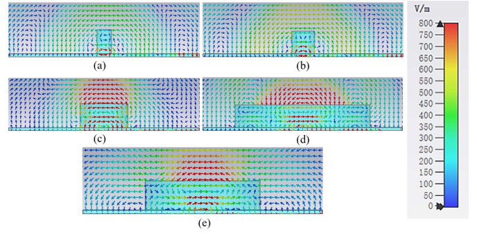
Fig. 2. Simulated electric field distribution of \text{HEM}_{11\delta+2} mode under different r/h ratios at 8 GHz frequency. (a) r = 2.7 mm, h = 8 mm. (b) r = 4 mm, h = 8 mm. (c) r = h = 8.9 mm. (d) r = 24 mm, h = 8 mm. (e) r = 17 mm, h = 8 mm.
