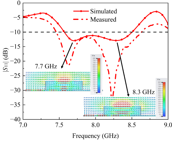
Fig. 4. Simulated and measured |S_{11}| and the electric field distributions at the two resonance frequencies.
