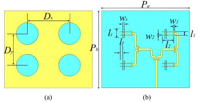
Fig. 7. Geometrical configuration of the DRA array. (a) Top view. (b) Bottom view. Design parameters: P_a = 136.4 , P_b = 120.05 , D_x = 65.4 , D_y = 49.05 , w_s = 3.3 , l_s = 10 , l_f = 5.15 , l_1 = 6.2 , w_1 = 0.9 , l_2 = 17.4 , and w_2 = 1 (unit: mm).
