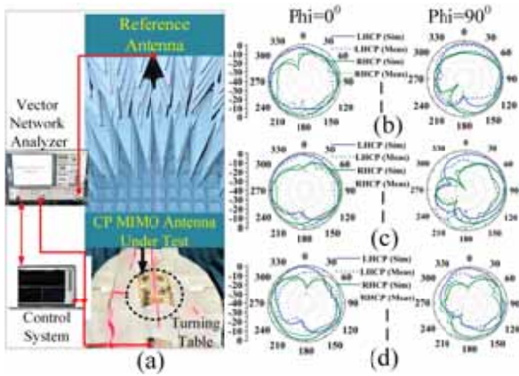
Fig. 5. (a) Testing setup of the proposed CP MIMO antenna in an anechoic chamber. Comparison of the simulated and measured LHCP and RHCP radiation patterns with the variation of phase angle \phi=0^\circ, 90^\circ at the frequency: (b) 2.4 GHz, (c) 3.5 GHz, and (d) 5.8 GHz.
