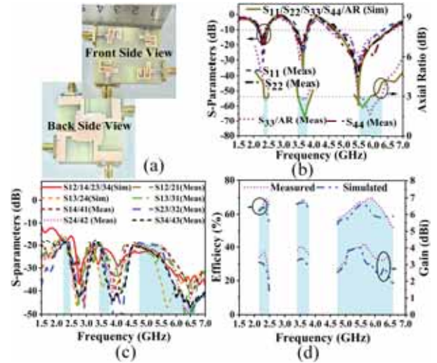
Fig. 4. (a) Front and back side views for fabricated four-port CP MIMO antenna prototype. (b) return loss (dB) and AR (dB), (c) transmission coefficient (dB), and (d) gain (dB), and efficiency (%) for simulated and measured proposed CP MIMO antenna.
