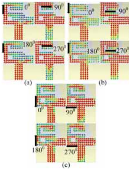
Fig. 3. The surface current distributions of port 1 and terminated other ports, with the orientation of different phase angles at the frequencies of (a) 2.4 GHz, (b) 3.5 GHz, and (c) 5.8 GHz.
