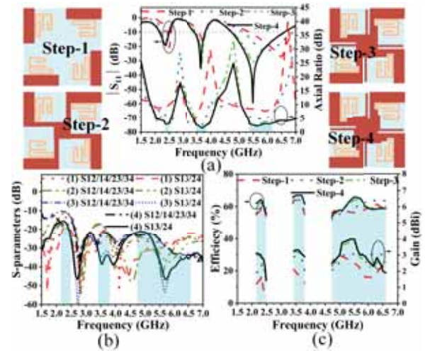
Fig. 2. (a) Simulated reflection coefficient (dB) and axial ratio (dB) results, along with its four steps design layout of the CP MIMO antenna, (b) simulated four steps design isolation (dB) plots, and (c) the four steps simulated gain (dBi) and efficiency (%) comparison plots.
