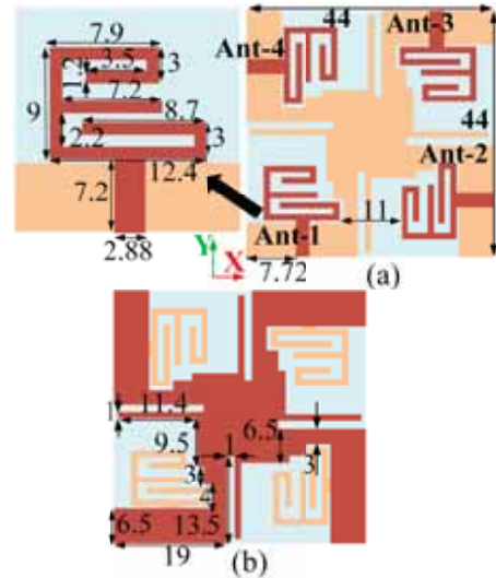
Fig. 1. Geometry of the proposed MIMO antenna: (a) front side view and (b) back side view (unit: mm)
