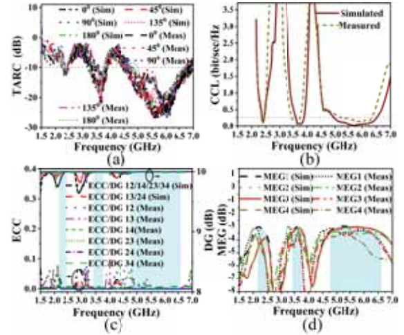
Fig. 6. Comparison of simulated and measured results of (a) TARC (dB), (b) CCL (bit/sec/Hz), (c) ECC and DG (dB), as well as (d) MEG (dB).
